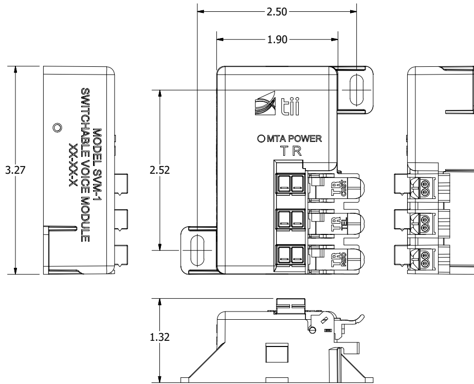
Dimensions are in Inches
