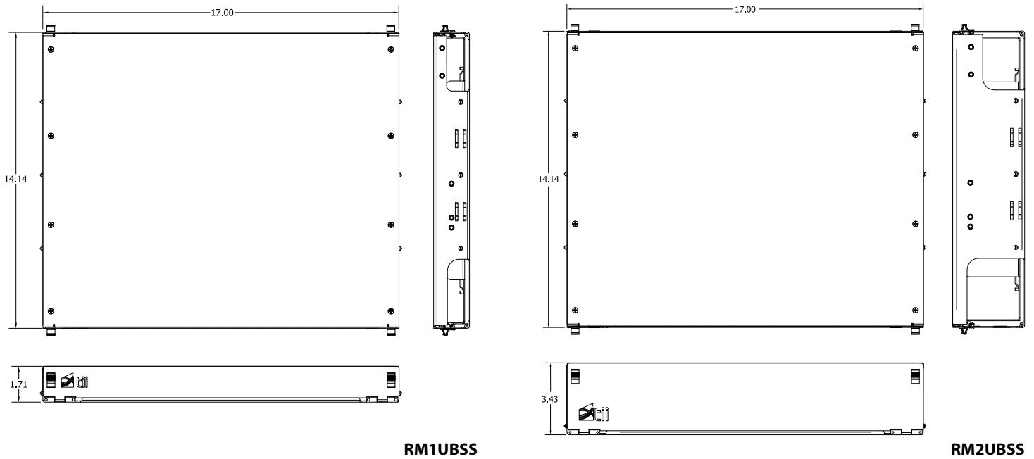
Dimensions are in Inches
